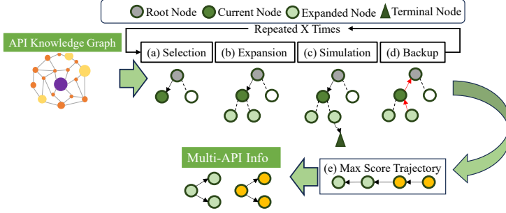
Fig. 6. Multi-API Non-Leaf Node Selection and Data Retrieval
