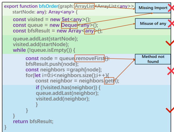
Fig. 1. The breadth-first traversal algorithm code under HarmonyOS generated by GPT-4o
